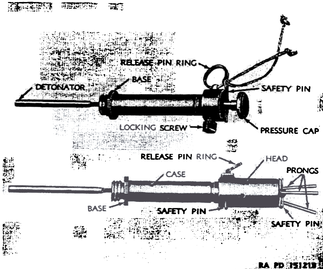
Figure 14. FUZES for mine, antipersonnel, M3.
